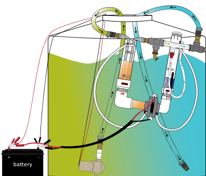
one-tank system
